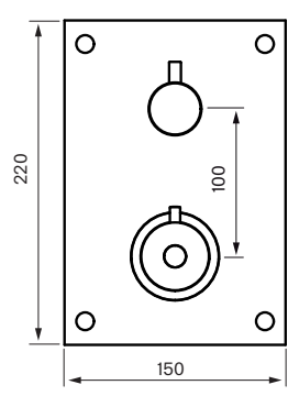
Mixer front view
