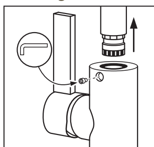
Figure 3B1
