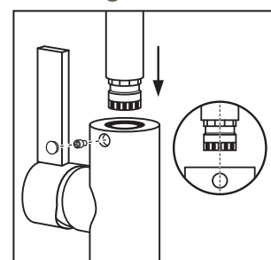
Figure 3B4
